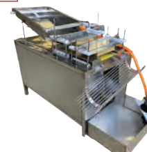
DOUBLE ROW QUAIL EGG PEELER
